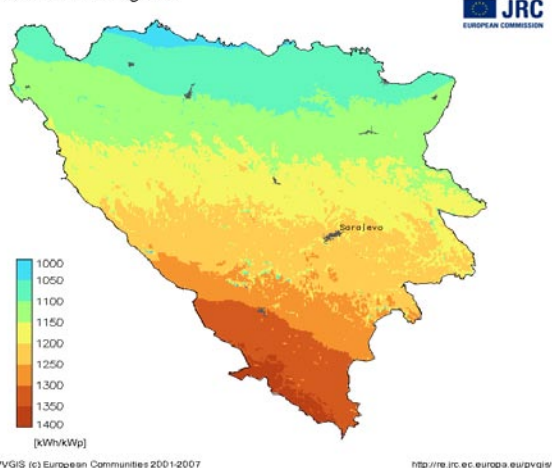
Yearly potential solar electricity generated by 1 kWp system with optimally tilted PV modules Bosnia and Herzegovina
